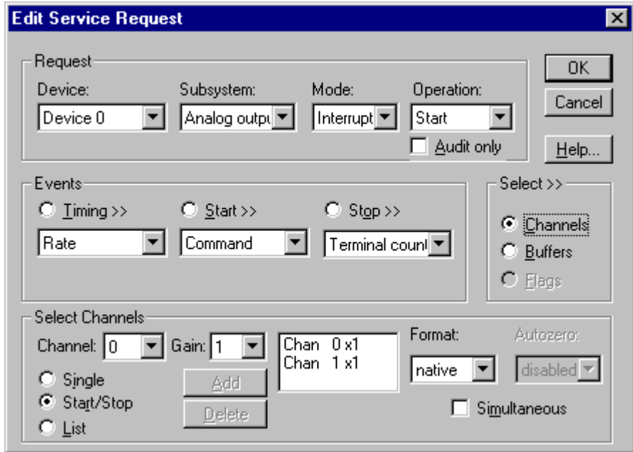
How to set up the KPCI-3108 Series for writing to a consecutive range of channels.
