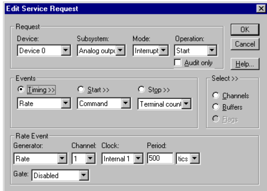
How to set up the KPCI-3108 Series for fixed rate writing using an internal clock.
