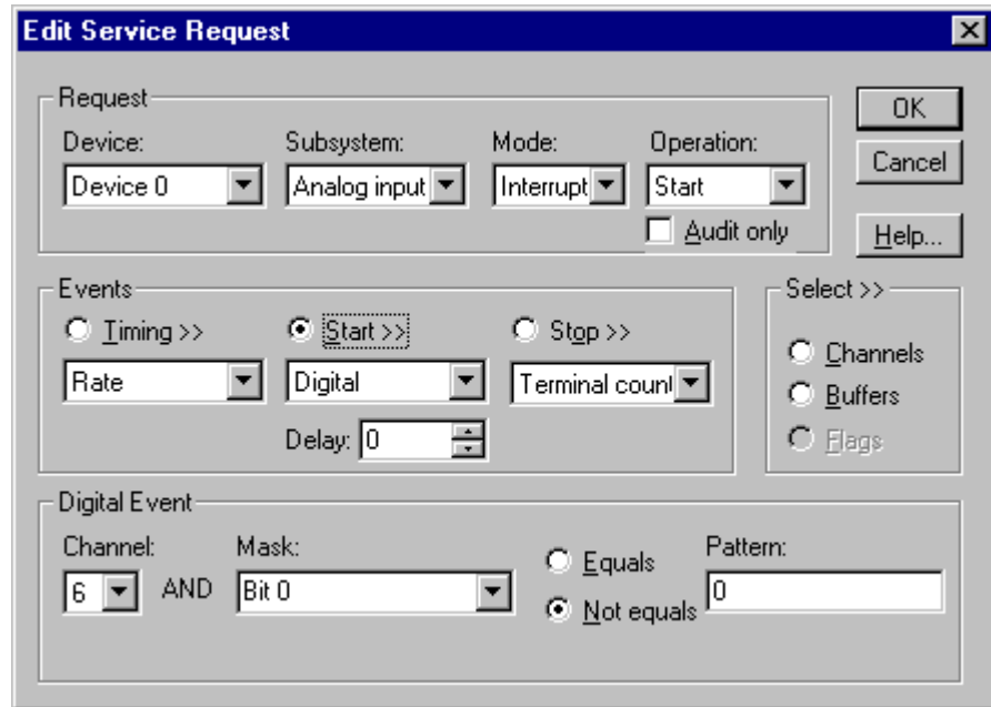
How to set up the KPCI-3108 Series for post-triggered analog input.
