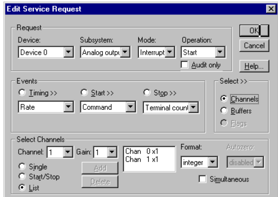
How to set up the KPCI-3108 Series to write to an arbitrary list of channels.
